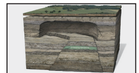
VT3 - Geology 101 Horst
