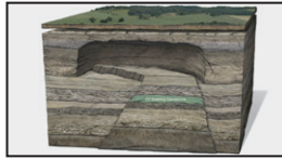
VT3 - Geology 101 Horst
