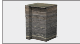
VT2 - Geology 101 Multi-Pay Sands
